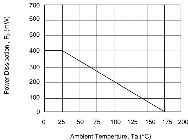
Derating Curve
